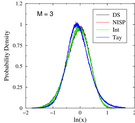
FIG. 3.19. Comparison of the PDF of \ln(x) generated with the TAYLOR series, integration and NISP/GH approaches to the directly sampled PDF for 3 d order PC representations. The integration approach matches the NISP/GH and directly sampled results, whereas the TAYLOR series does not converge.
