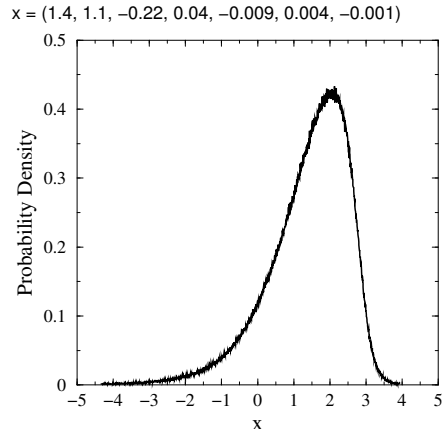
FIG. 3.9. PDF of the variable x(1.4, 1.1, -0.22, 0.04, -0.009, 0.004, -0.001)
