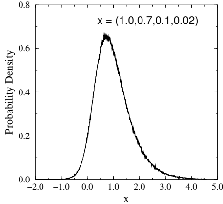
FIG. 3.1. PDF of the variable x with the PC expansion x(1.0, 0.7, 0.1, 0.02)
