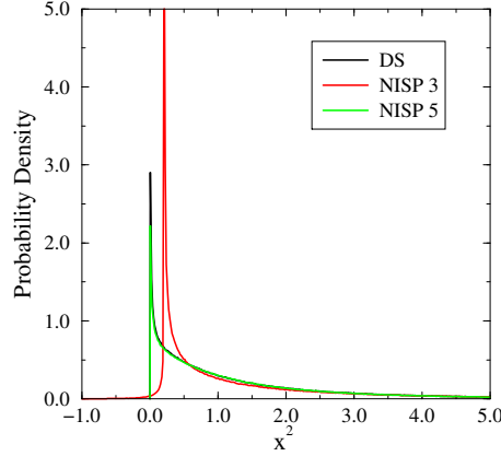
FIG. 3.2. PDF of x^2 as obtained from direct sampling (DS), as well as from NISP/GH with both 3 rd and 5 th order PC. The 5 th order PC expansion represents the exact PDF well.
