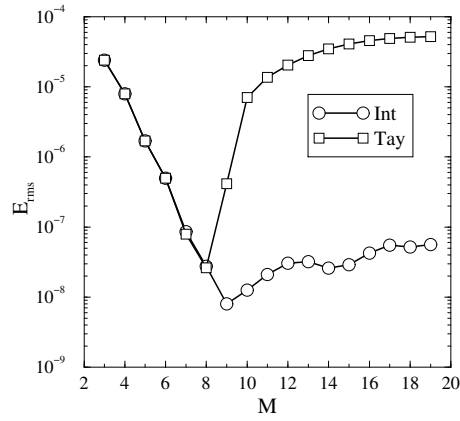
FIG. 3.15. RMS difference between the PC coefficients of \ln(x) for the TAYLOR series and integration approaches compared to the NISP/GH method, as a function of the order M of the expansion used. The TAYLOR series breaks down for M > 8 . The integration approach gets closer to the NISP/GH results up to order 9 but then levels off.
