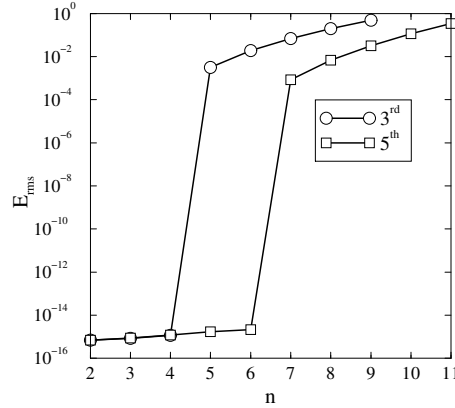
FIG. 3.4. Root-mean-squared error in the PC coefficients of x^n obtained with a 3 rd and a 5 th order PC pseudo-spectral method. The error increases dramatically for powers of x that are more than one larger than the order of the PC expansions.
