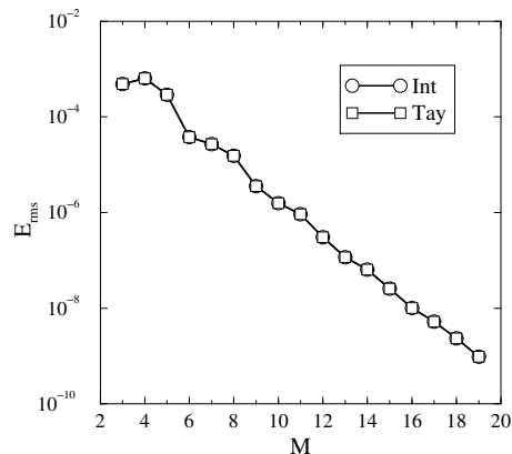
FIG. 3.7. Root-mean-squared difference between the PC coefficients of \exp(x) for the TAYLOR series and integration approaches compared to the NISP/GH method, as a function of the order M of the expansion used. Both TAYLOR series and the integration approach give the same results.
