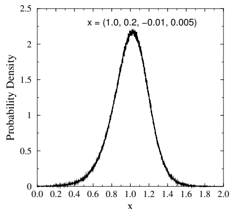
FIG. 3.6. PDF of the variable x given by the PC expansion x(1.0, 0.2, -0.01, 0.005)
