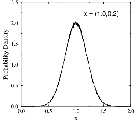
FIG. 3.3. PDF of the variable x given by the PC expansion x(1.0,0.2)
