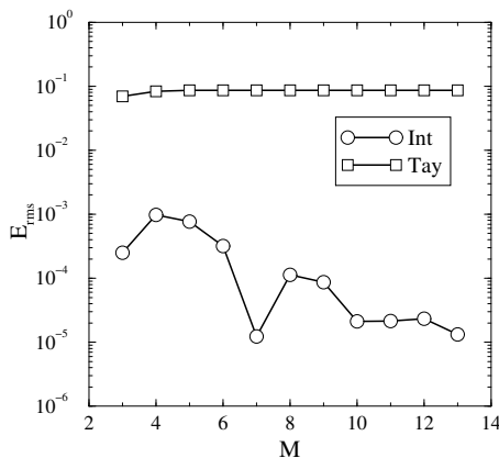
FIG. 3.18. RMS difference between the PC coefficients of \ln(x) for the TAYLOR series and integration approaches compared to the NISP/GH method, as a function of the order M of the expansion used. The TAYLOR series is not convergent for this case but the integration approach gives results that generally improve for increasing M .
