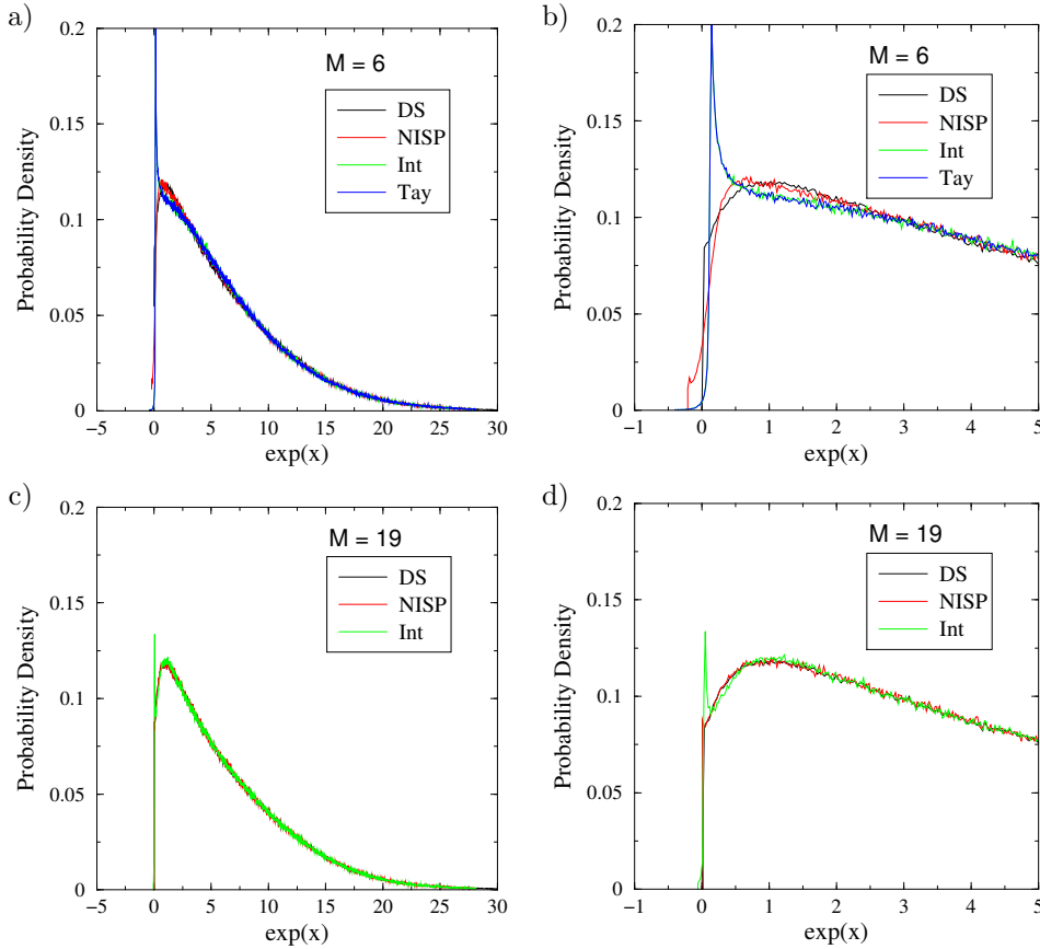
FIG. 3.11. Comparison of the PDF of \exp(x) generated with the TAYLOR series, integration and NISP/GH approaches to the directly sampled PDF: a) Approximations with 6 th order PC expansions; b) Same, but zoomed in on the origin; c) Approximations with 19 th order PC expansions; d) Same, but zoomed in on the origin.
