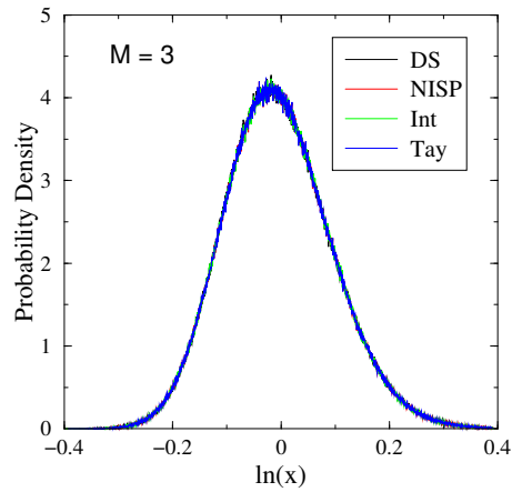
FIG. 3.16. Comparison of the PDF of \ln(x) generated with the TAYLOR series, integration and NISP/GH approaches to the directly sampled PDF for 3 rd order PC representations.
