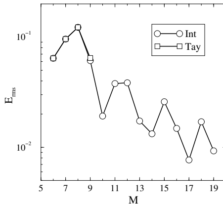
FIG. 3.10. Root-mean-squared difference between the PC coefficients of \exp(x) for the TAYLOR series and integration approaches compared to the NISP/GH method, as a function of the order M of the expansion used. The TAYLOR series breaks down for M > 9 whereas the integration approach gets closer to the NISP/GH results for increasing M .
