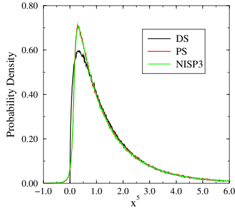
FIG. 3.5. PDF of x^5 as obtained by direct sampling (DS), pseudo-spectral (PS) calculation with 3 rd order PC, as well as the sampling of the NISP/GH result truncated after the 3 rd . The low order PC expansion results in finite probabilities for negative values of x^5 .
