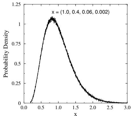
FIG. 3.17. PDF of the PC variable x(1.0, 0.4, 0.06, 0.002)
