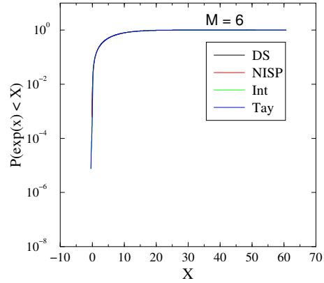
FIG. 3.12. Comparison of the tails of the CDF P(\exp(x) < X) generated with the TAYLOR series, integration and NISP/GH approaches to the directly sampled results.
