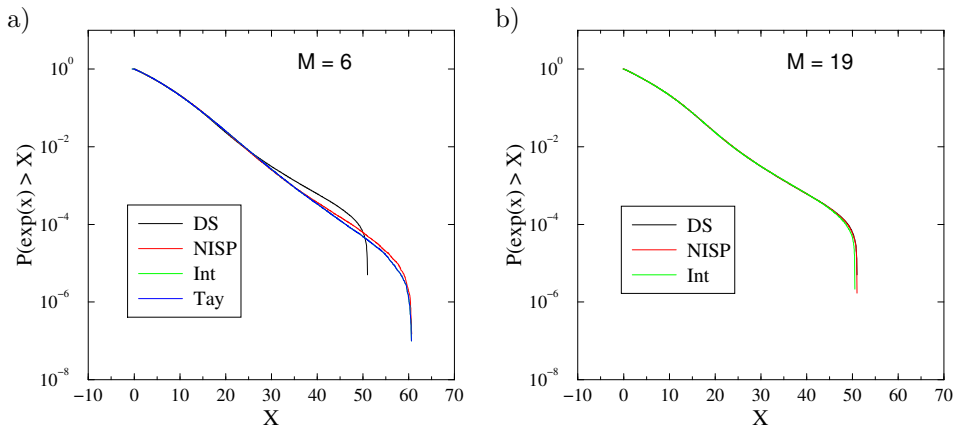
FIG. 3.13. Comparison of the tails of the CDF P(\exp(x) > X) generated with the TAYLOR series, integration and NISP/GH approaches to the directly sampled results: a) Approximations with 6 th order PC expansions; b) Approximations with 19 th order PC expansions.
