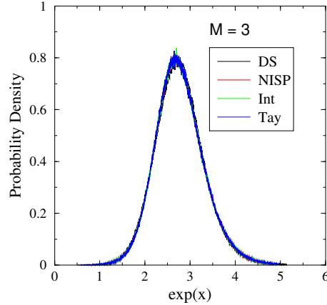
FIG. 3.8. Comparison of the PDF of \exp(x) as generated with the different methods using 3 rd order PC representations. All methods give the same result.
